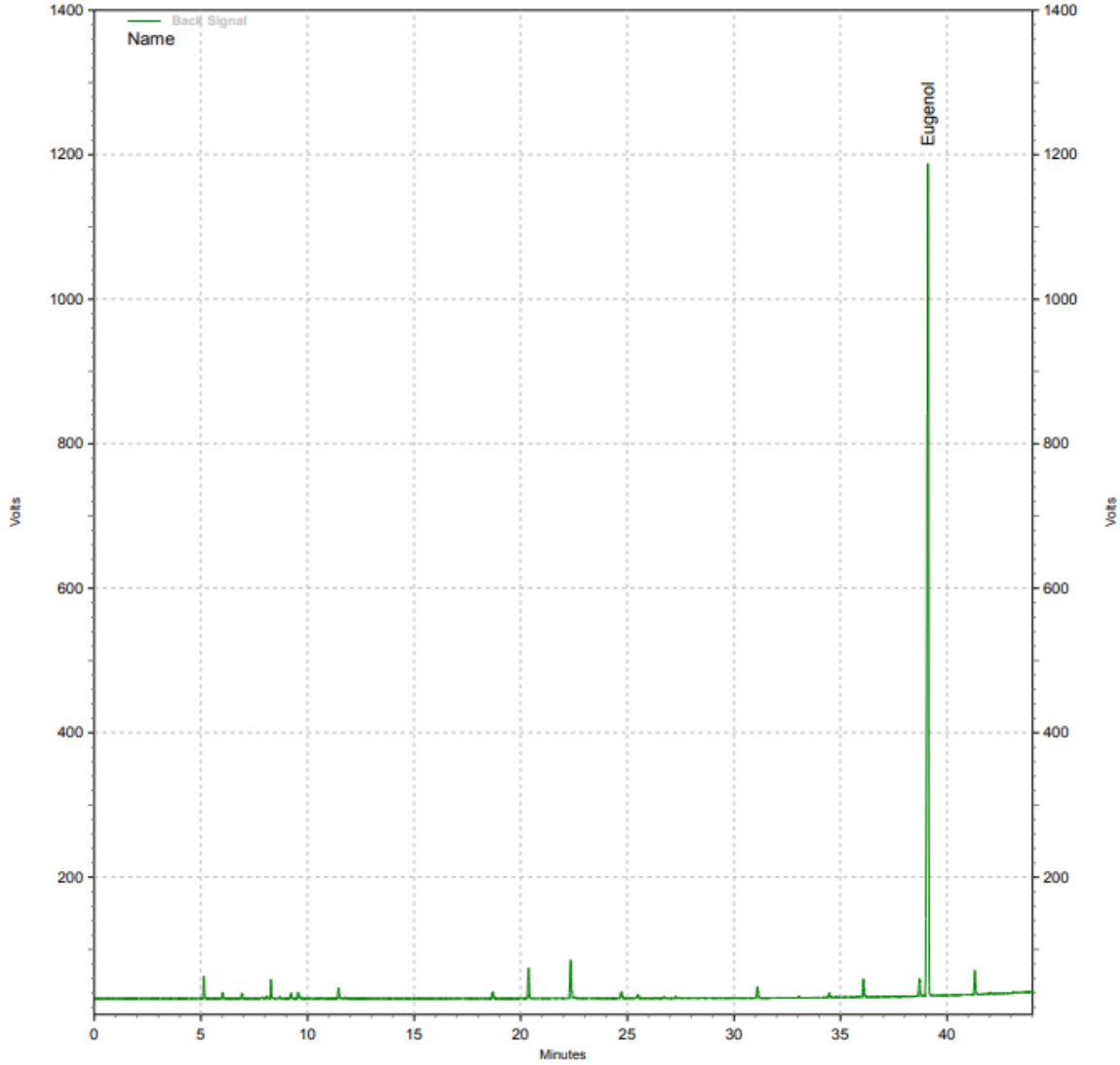
Representative Chromatogram of Cinnamon Leaf Oil (2342050803).
