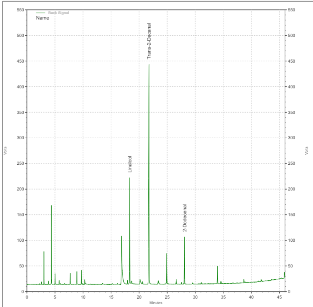
Representative Chromatogram of Coriander Leaf Oil (2442032918).
