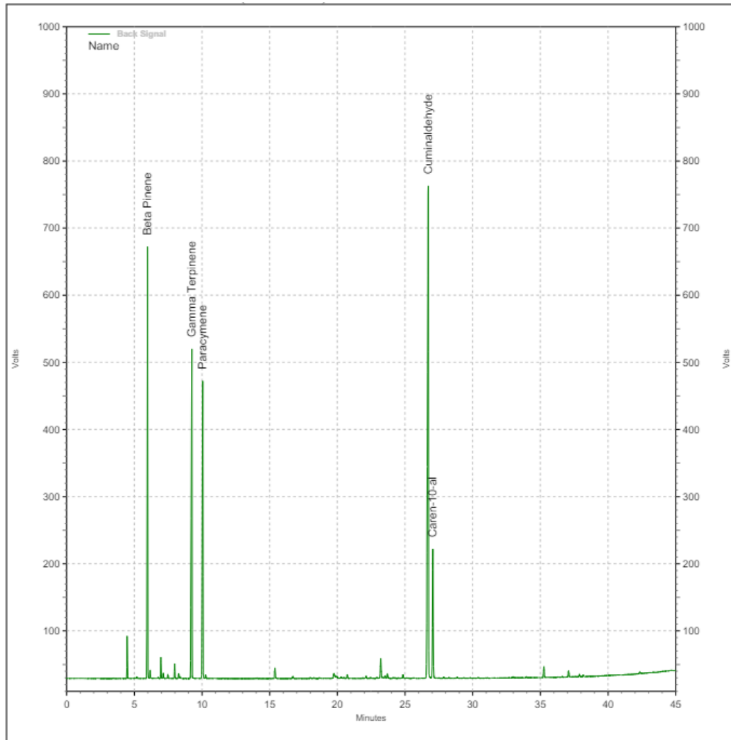
Representative Chromatogram of Cumin Seed Oil (2442021501).
