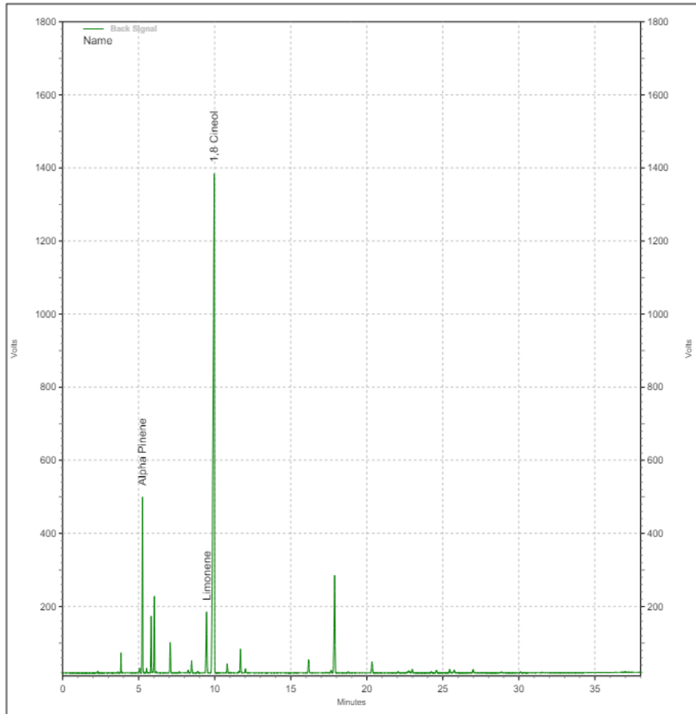
Representative Chromatogram of Eucalyptus Oil (G) (2342032501).
