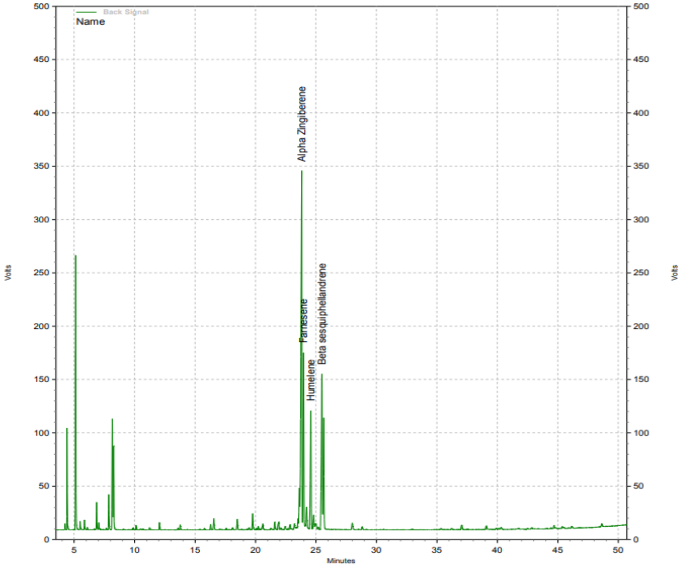
Representative Chromatogram of Ginger Oil (2442030708).
