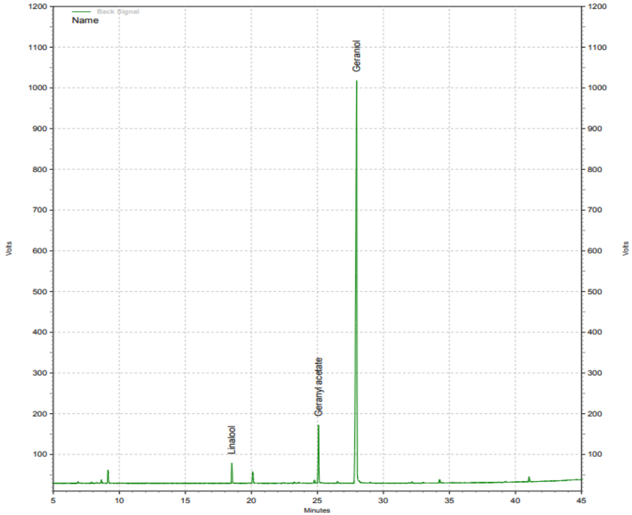
Representative Chromatogram of Palmarosa Oil (2442030404).
