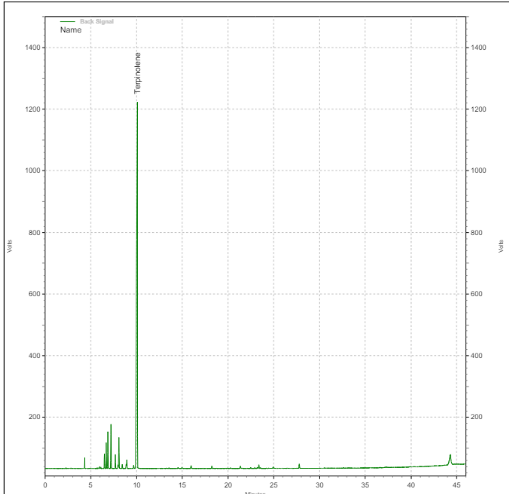
Representative Chromatogram of Turmeric Leaf Oil (2442040207).
