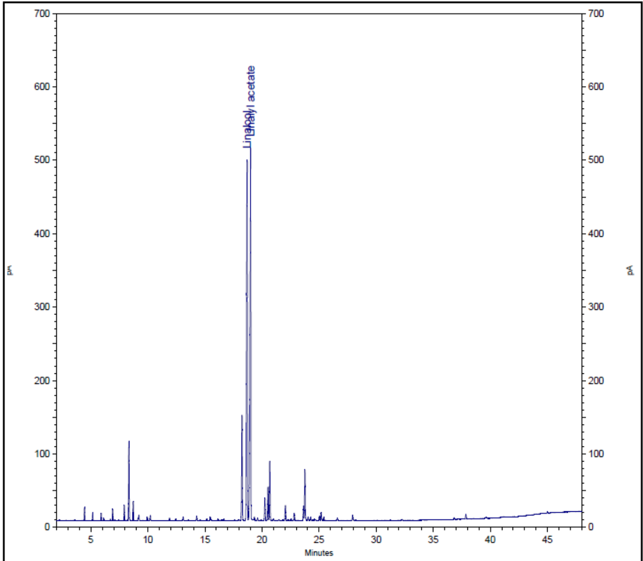
Representative Chromatogram of Lavandin Oil (Grasso) (2442022110).
