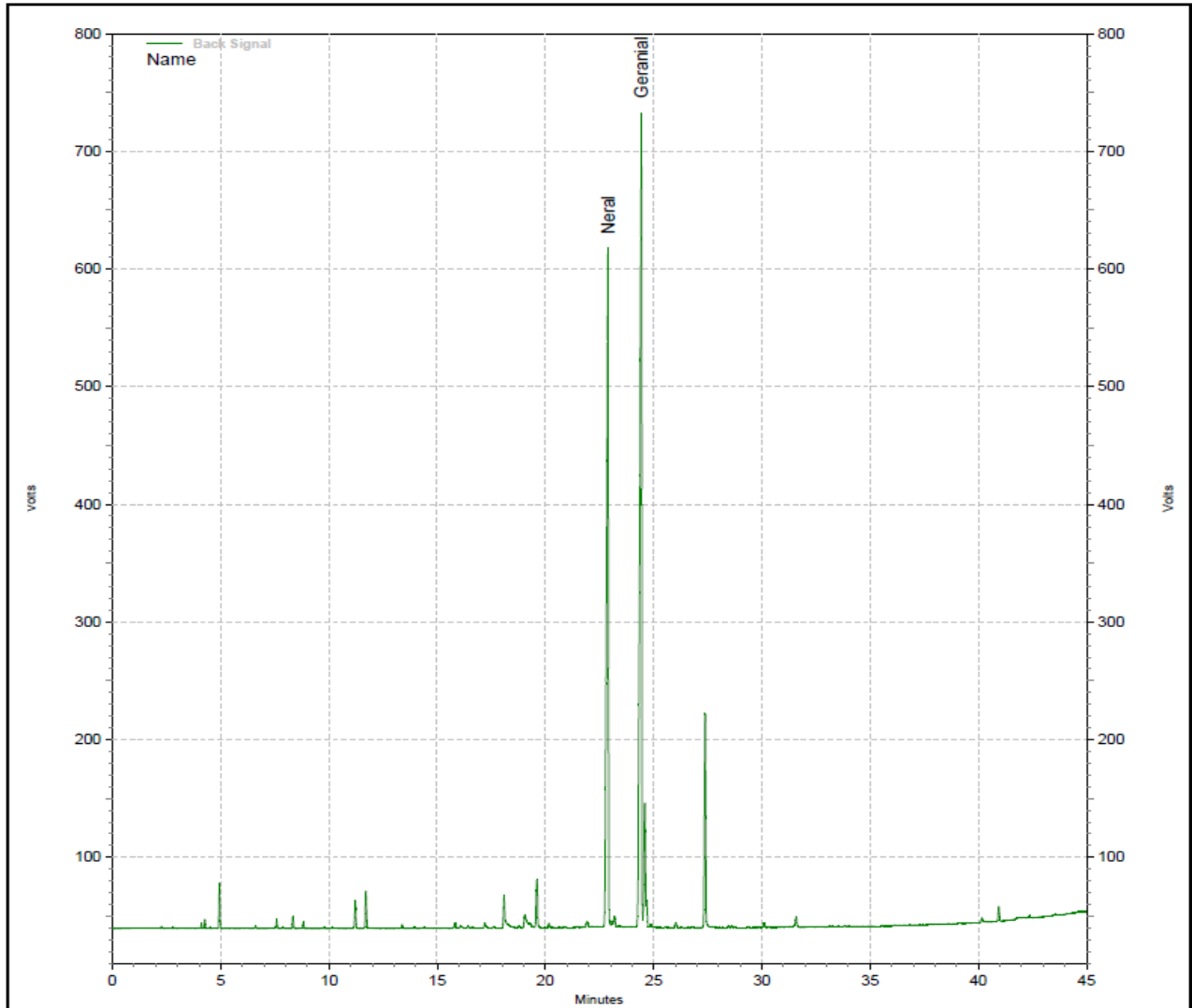
Representative Chromatogram of Lemon Grass Oil (2442042501).
