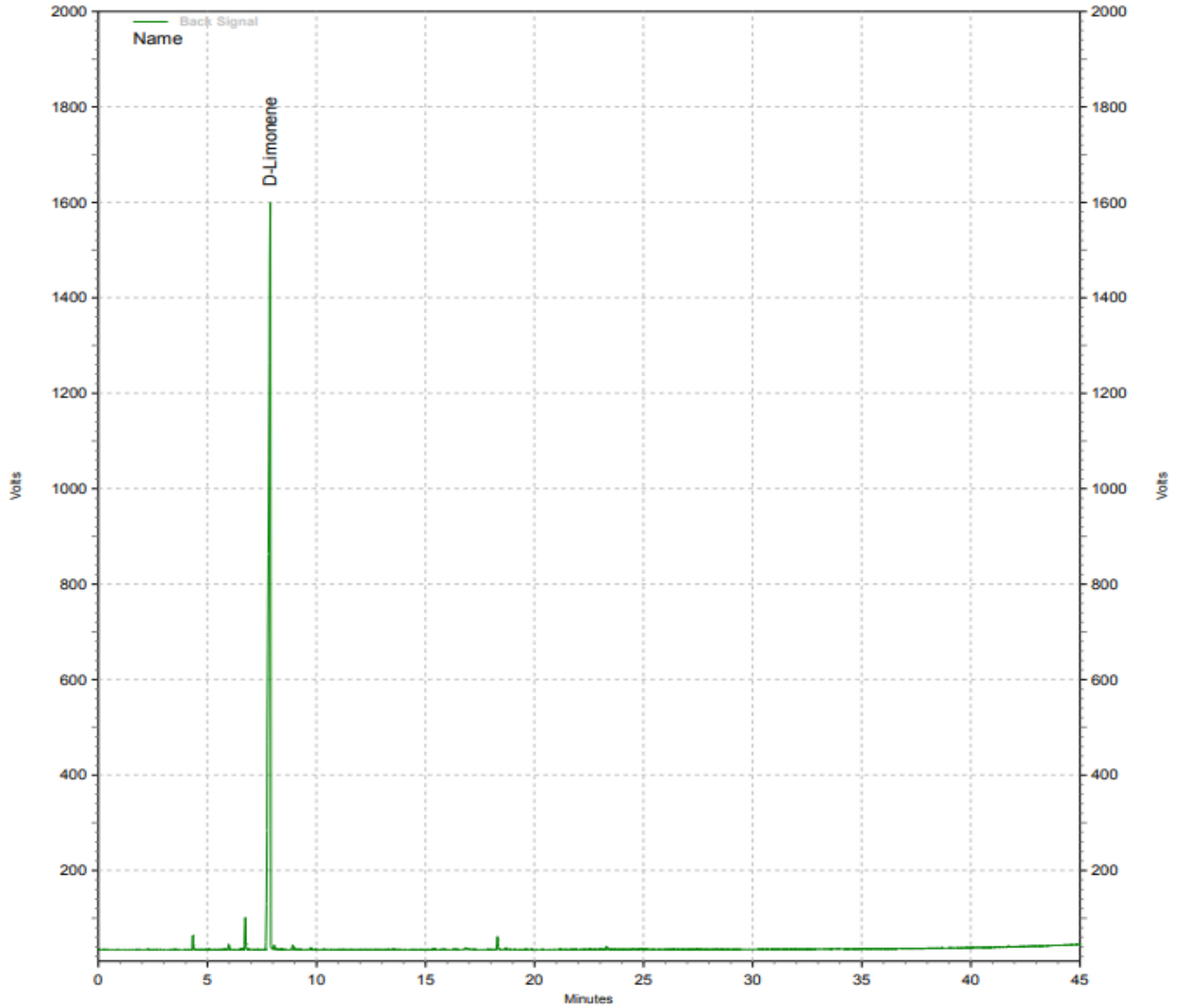
Representative Chromatogram of Orange Oil (2442032919).
