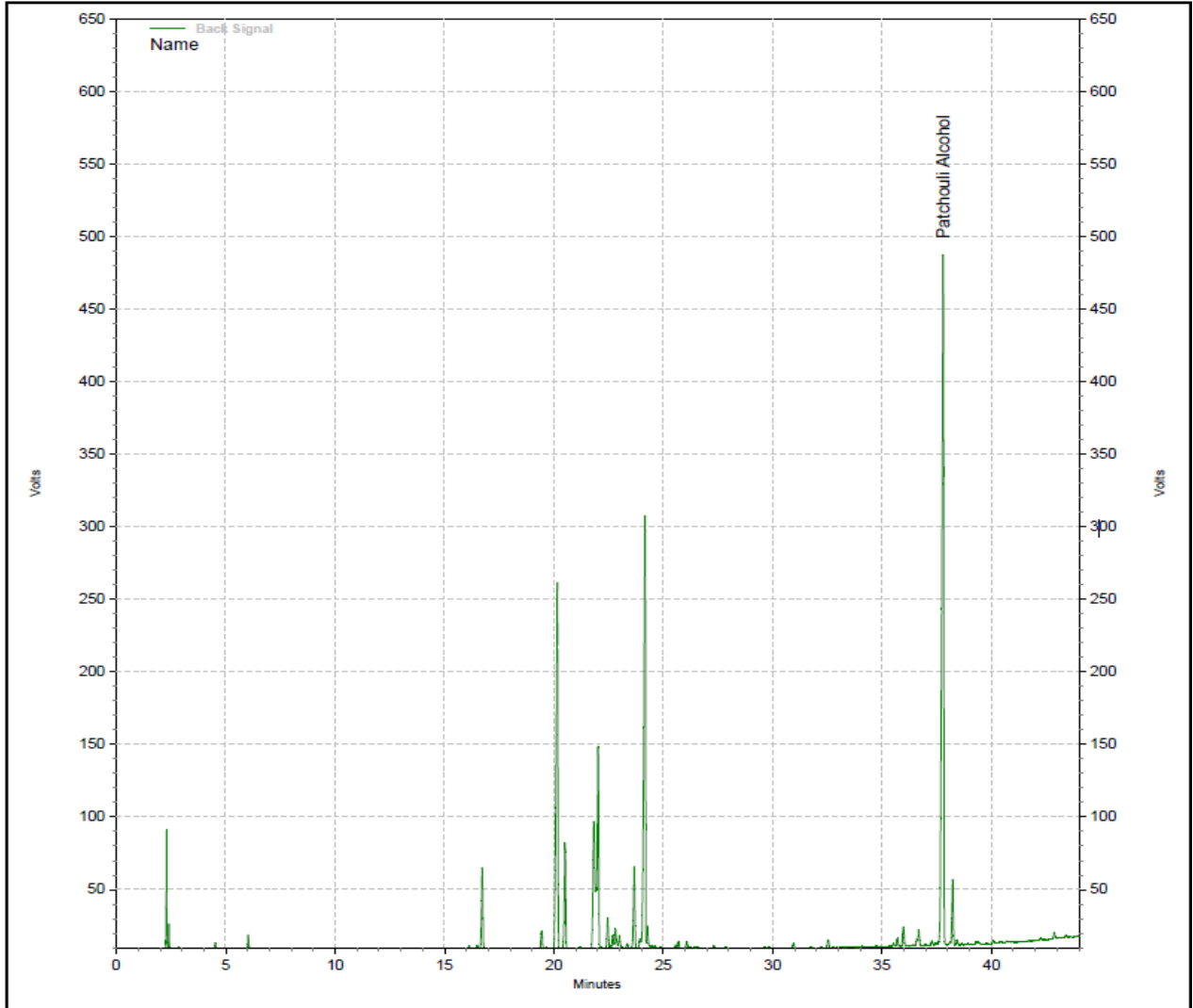
Representative Chromatogram of Patchouli Oil (2442012506).
