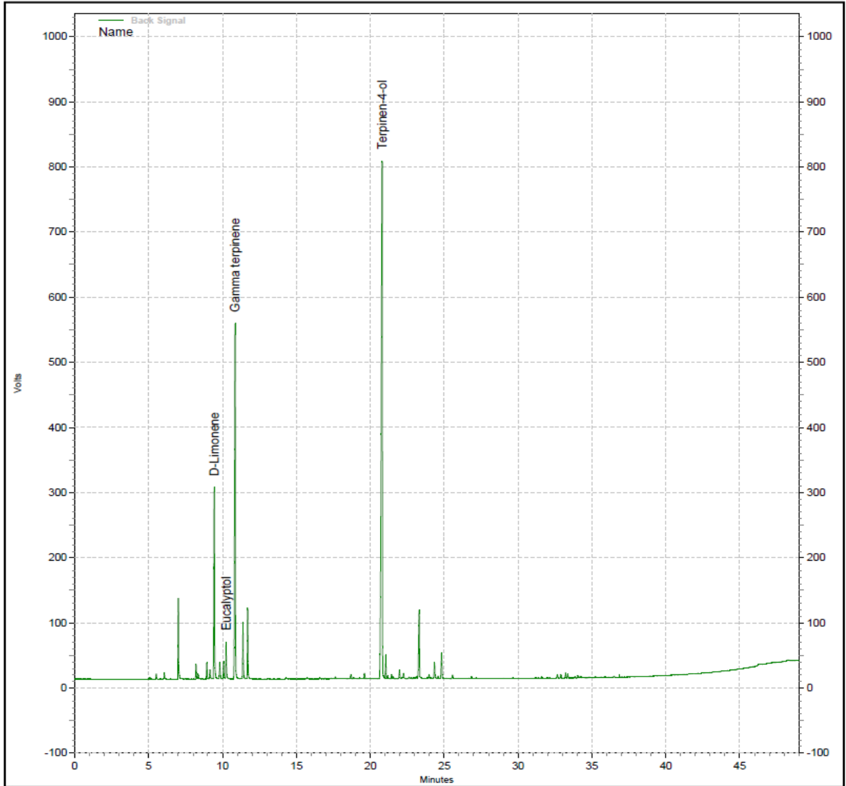
Representative Chromatogram of Tea Tree Oil (Australian) (2242021402).
