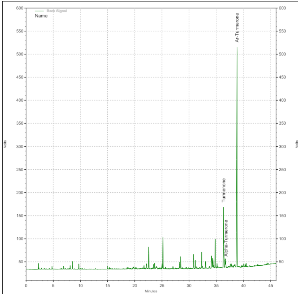
Representative Chromatogram of Turmeric Root Oil (2442032313).
