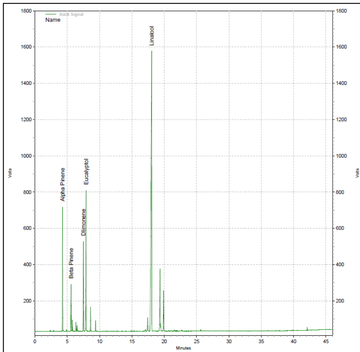
Representative Chromatogram of Hyssop Oil (2442052818).
