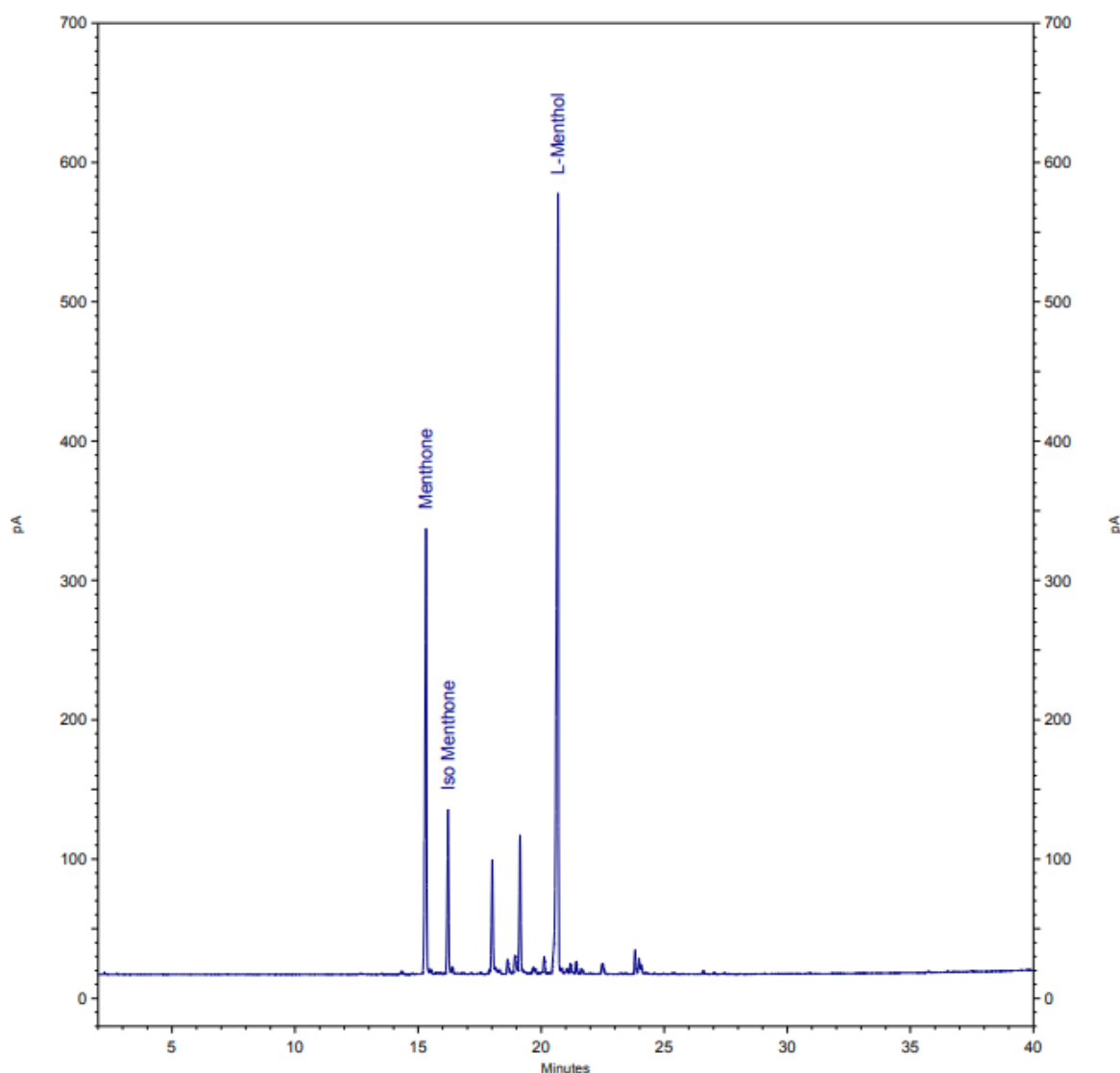
Representative Chromatogram of Peppermint Oil (2442091602).
