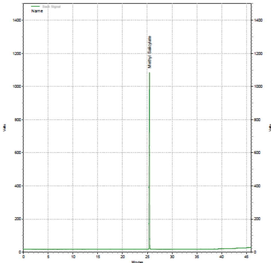
Representative Chromatogram of Wintergreen Oil (2442062607).
